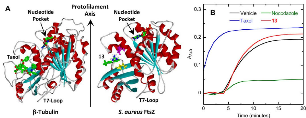
Figure 11. (A) Comparison of the crystal structure of the \beta -tubulin–taxol complex (PDB 1JFF) 59 with the homology model of SaFtsZ in complex with 13. The proteins, nucleotides, and compounds are depicted as described in Figure 6A. The orientation of protofilament growth is indicated. (B) Comparison of the impact of 13 and the antineoplastic drugs paclitaxel (taxol) and nocodazole on the polymerization of microtubule-associated protein (MAP)-rich porcine \beta -tubulin (70% \beta -tubulin, 30% MAPs) at 37 °C. The time-dependent A_{340} profiles of 2 mg/mL porcine \beta -tubulin are presented in the presence of vehicle (DMSO) only (black), 40 \mu\text{g/mL} 13 (red), 25 \mu\text{g/mL} taxol (blue), or 10 \mu\text{g/mL} nocodazole (green). Experimental conditions for the tubulin polymerization studies were 80 mM PIPES-NaOH (pH 7.0), 2 mM \text{MgCl}_2 , 1 mM EGTA, and 1 mM GTP.
