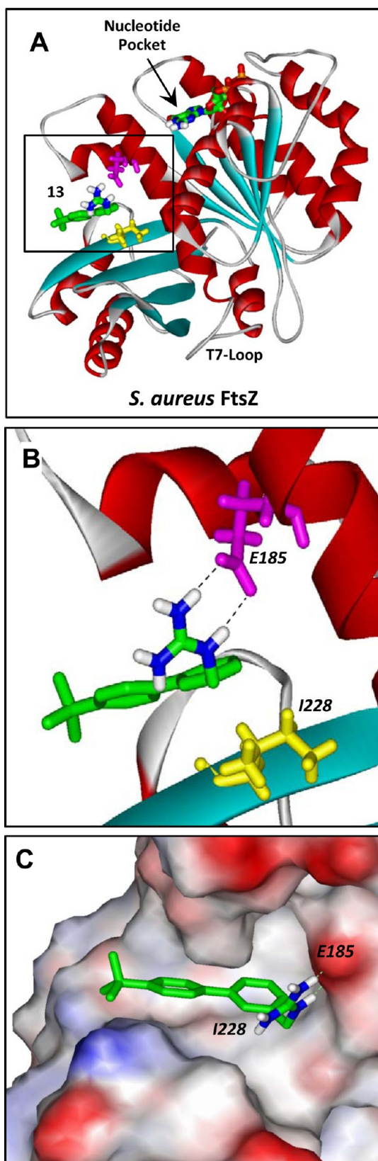
Figure 6. Structural homology model of SaFtsZ in complex with 13 derived as detailed in Experimental Section. (A) SaFtsZ is schematically depicted according to its secondary structural elements ( \alpha -helices in red, \beta -strands in cyan, and loops in gray), with the GTP binding pocket and T7 loop (which is involved in nucleotide hydrolysis when the proteins are polymerized) indicated. The 13 -FtsZ complex shown reflects the highest scoring complex obtained using the Autodock Vina
