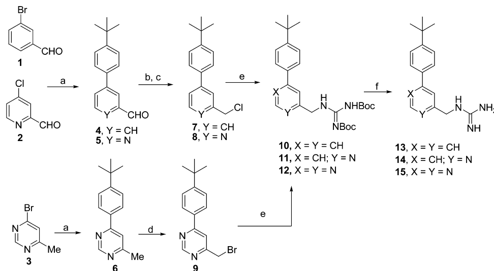
Scheme 1. Methods Used in the Preparation of the Guanidinomethyl Biaryl Analogues 13–15 a
