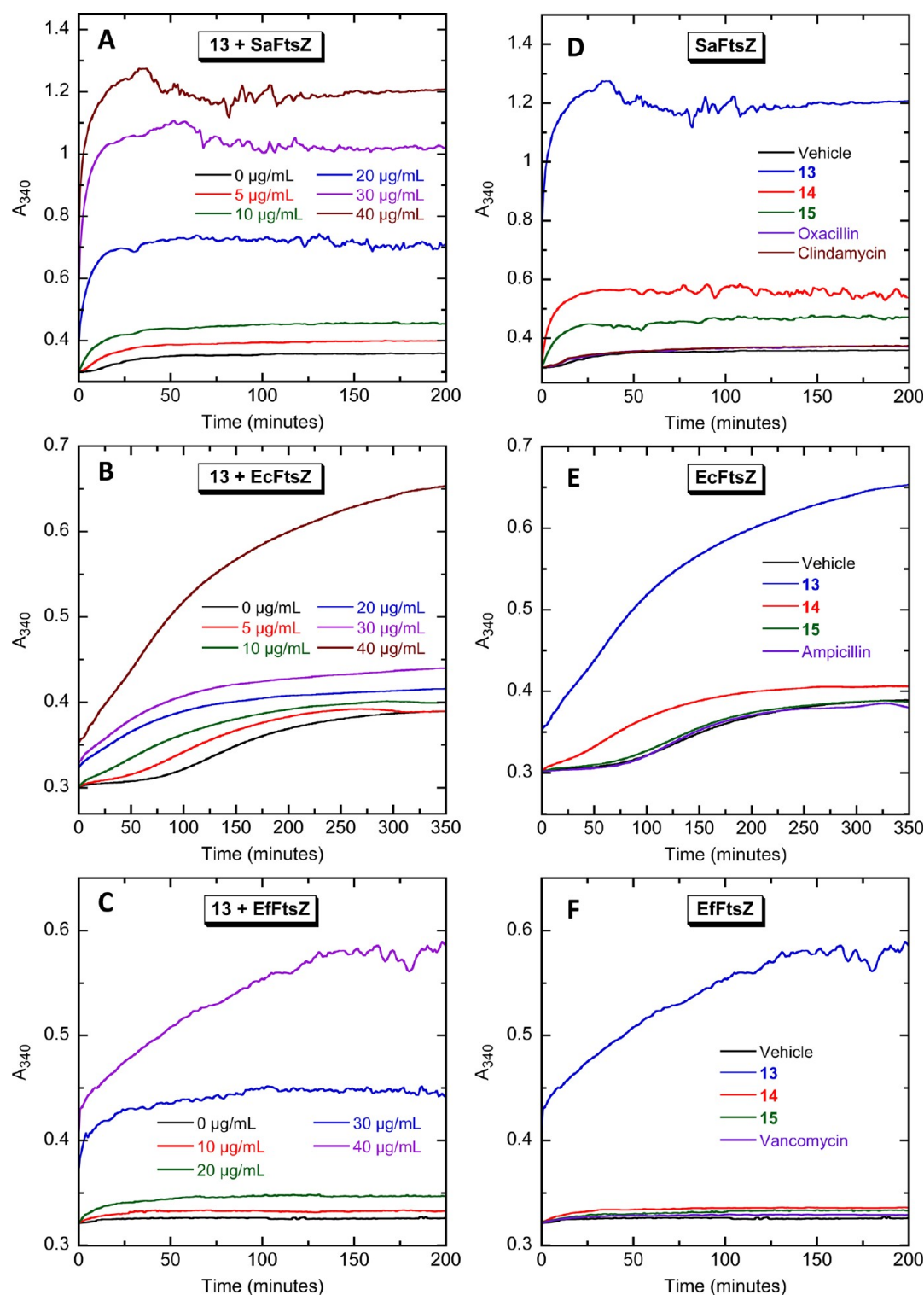
Figure 3. Concentration dependence and structure–activity relationship of the impact of the biaryl compounds on the polymerization of SaFtsZ (A and D), EcFtsZ (B and E), and EffFtsZ (C and F), as determined by monitoring time-dependent changes in absorbance at 340 nm ( A_{340} ) at 25 °C. (A–C) The time-dependent A_{340} polymerization profiles of each target FtsZ in the presence of 13 at the indicated concentrations. (D–F) Time-dependent A_{340} polymerization profiles of each target FtsZ in the presence of vehicle (DMSO) only or 40 \mu\text{g/mL} of 13 , 14 , 15 , or the indicated comparator drugs. Experimental conditions for all the FtsZ polymerization studies were 10 \mu\text{M} protein, 50 mM Tris-HCl (pH 7.4), 50 mM KCl, 2 mM magnesium acetate, 1 mM \text{CaCl}_2 (for SaFtsZ) or 10 mM \text{CaCl}_2 (for EcFtsZ and EffFtsZ), and 1 mM GTP.
