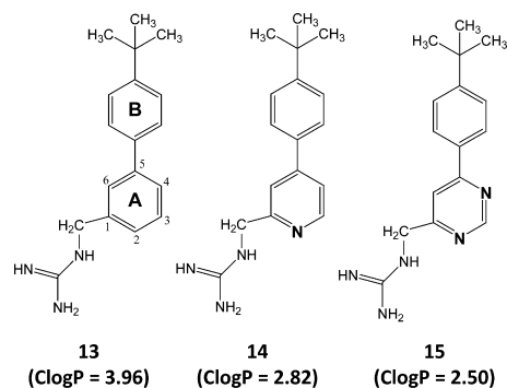
Figure 1. Chemical structures and calculated lipophilicities (ClogP) of 13–15. The indicated ClogP values were calculated using the weighted method (VG = KLOP = PHYS = 1) in the Marvin 5.7 Software Suite (ChemAxon, Ltd.), with Cl - and Na + /K + concentrations being set at 0.1 mol/dm 3 . The atomic numbering and ring lettering are indicated in the structure of 13 .
