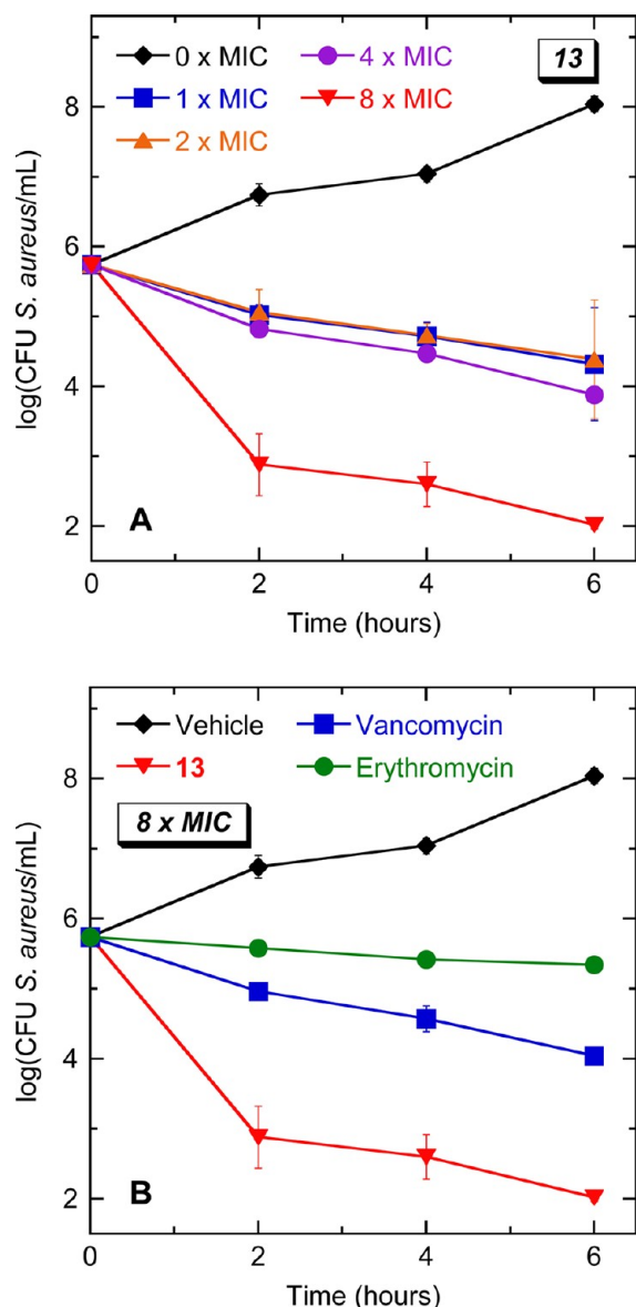
Figure 9. Time–kill curves for S. aureus 8325-4 (MSSA). Each data point reflects the average of two independent measurements, with the error bars reflecting the standard deviation from the mean. (A) Bacteria were treated with vehicle (DMSO) only or 13 at concentrations ranging from 1 to 8 × MIC (1 to 8 μg/mL). (B) Bacteria were treated with vehicle only, 13, vancomycin, or erythromycin. When present, all agents were used at a concentration corresponding to 8 × MIC.
