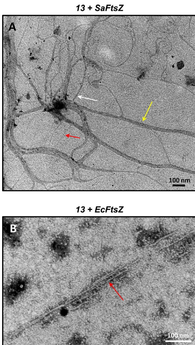
Figure 4. Transmission electron micrographs of 13-induced filaments of (A) SaFtsZ and (B) EcFtsZ. Polymerization of the proteins was induced by addition of 20 \mu\text{g}/\text{mL} 13 under the experimental conditions described in the legend to Figure 3. The filaments were negatively stained with a solution of 1% phosphotungstic acid (PTA) and visualized at 80 kV on a Philips CM12 transmission microscope interfaced with an AMT XR111 camera. The red, white, and yellow arrows in panel A highlight filaments 5, 11, and 25 nm wide, respectively. The red arrow in panel B highlights a 5 nm wide filament.
