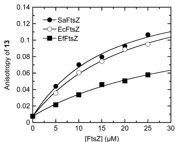
Figure 2. Fluorescence anisotropies of 5 \mu\text{M} 13 as a function of increasing concentrations of SaFtsZ (●), EcFtsZ (○), or EffFtsZ (■). The solid lines reflect the nonlinear least-squares fits of the data with eq 1. Experiments were conducted at 25 °C in solution containing 50 mM Tris-HCl (pH 7.4), 50 mM KCl, and 2 mM magnesium acetate.
